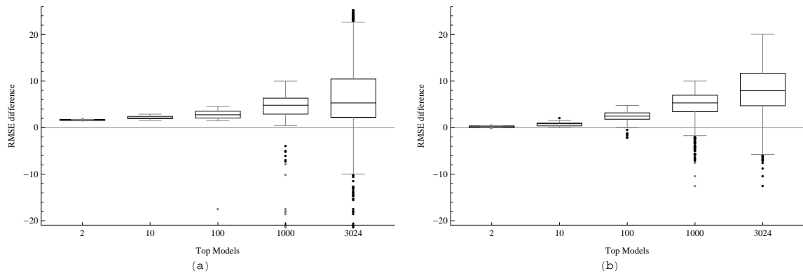
Figure C.9: Distribution of the model-wise differences of RMSE between ProBMoT/ALG and ProBMoT/DASA for all automated modeling tasks for the Glumsø domain. (a) Glumsø '73; (b) Glumsø '74.
