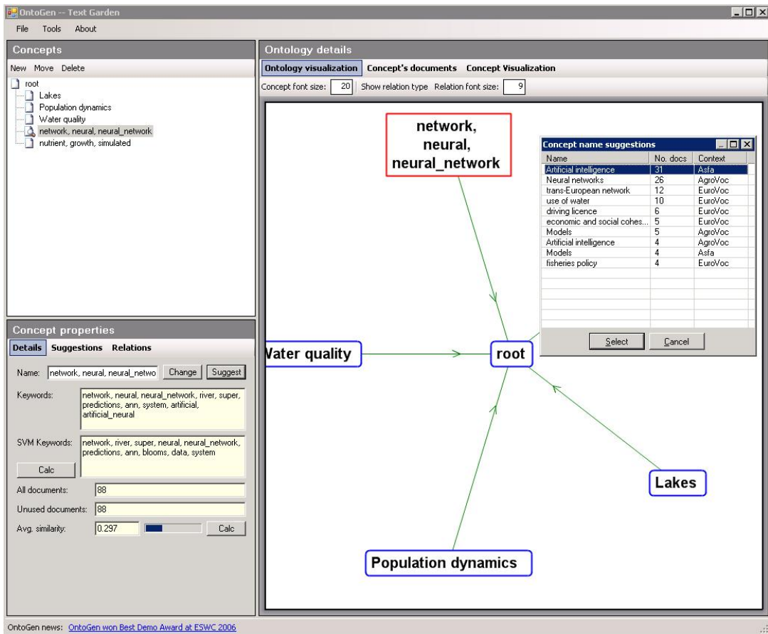
Figure 1: A screenshot of OntoGen when used to structure the abstracts of recent issues of the Ecological Modelling journal. Contexts are provided by three ontologies: AgroVoc , ASFA , and EuroVoc . Some concept names were already derived from contextual suggestions ( Water quality , Population dynamics , Lakes ) and the user inspects current suggestions for the top node ( network, neural, neural_network ). The system provides two sensible suggestions: Artificial Intelligence (from ASFA ) and Neural networks (from AgroVoc ), while the third suggestion: trans-European network (from EuroVoc ) probably makes less sense.
