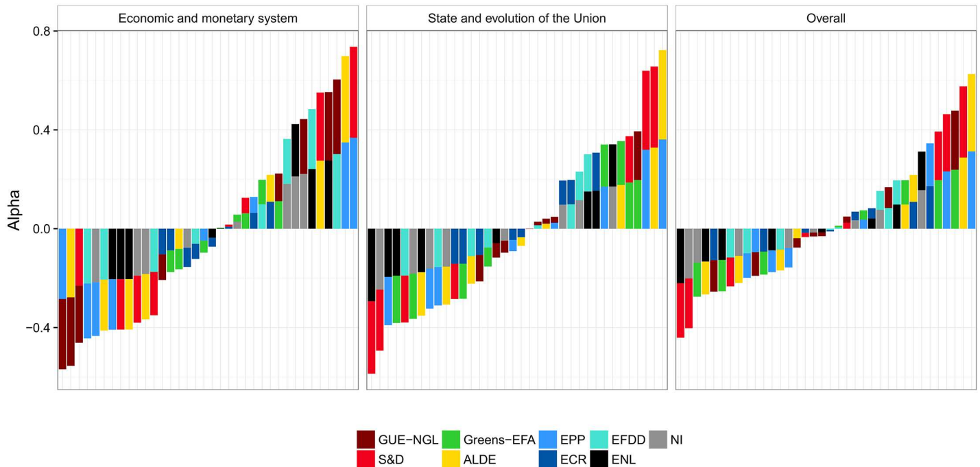
Fig 6. Coalitions between political groups in terms of RCVs as measured by Krippendorff's Alpha . For nine groups, there are 36 pairs for which we measure their (dis)agreement. Positive values of Alpha indicate co-voting agreement, negative values correspond to systematic disagreement, while Alpha = 0 indicates co-voting by chance. The average Alpha across all 36 pairs is 0.02, close to co-voting by chance. Note, however, that Alpha considers just yes/no votes, and ignores abstentions.
