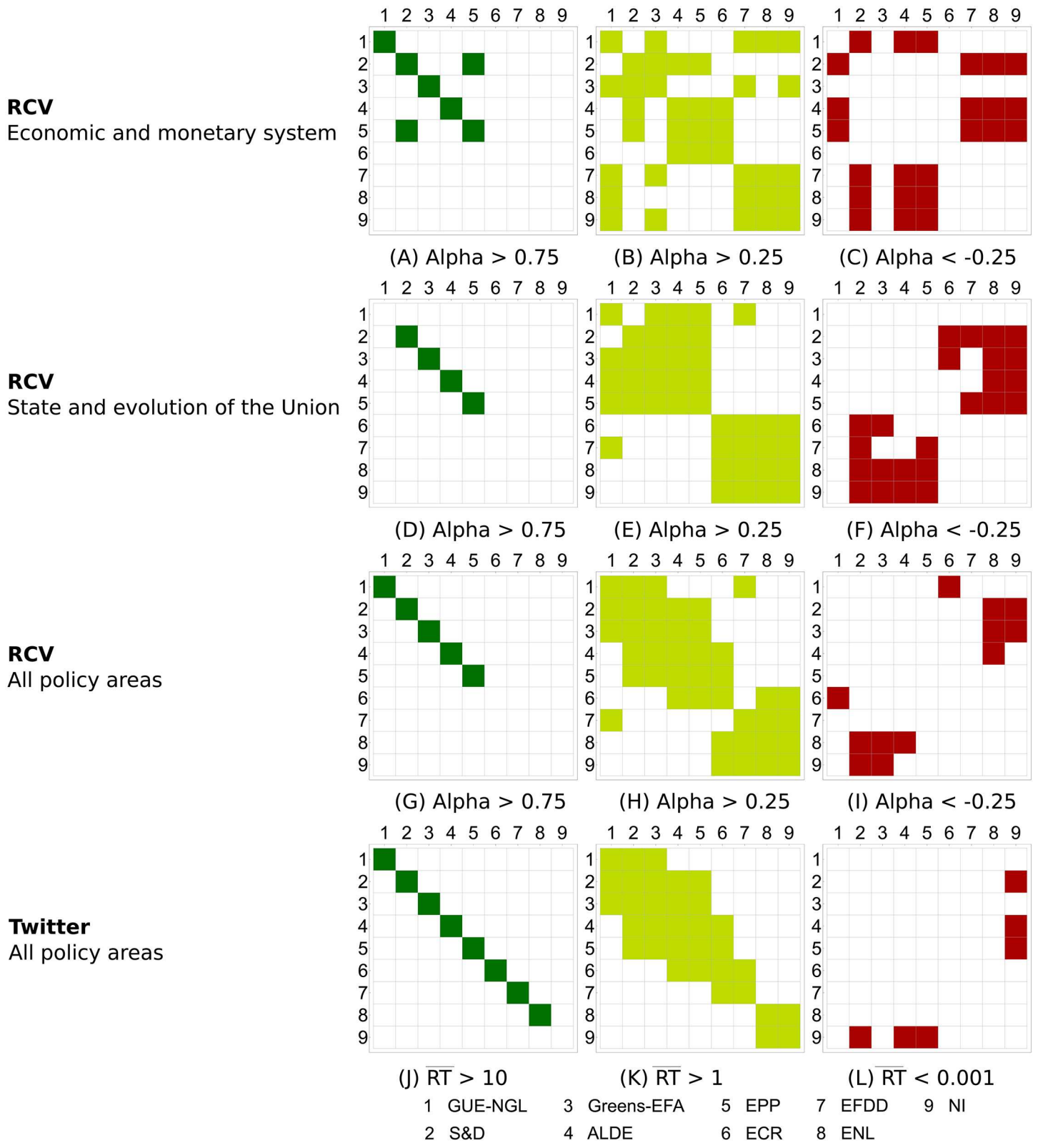
Fig 9. Formation of coalitions ( \text{Alpha} > 0 ) and oppositions ( \text{Alpha} < 0 ) in terms of the co-voting agreement (RCV). In the case of Twitter (the bottom charts), coalitions are indicated by higher average retweets ( \overline{\text{RT}} ), and oppositions by lower average retweets.
