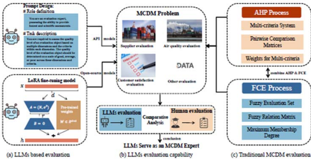
Figure 1: Overview of the proposed LLMs-based MCDM Framework. (a) The API models and the LoRA fine-tuned models are evaluated separately for MCDM. (b) Comparative analysis of the two sets of evaluation results. (c) Conducting MCDM evaluation combining traditional Models.
