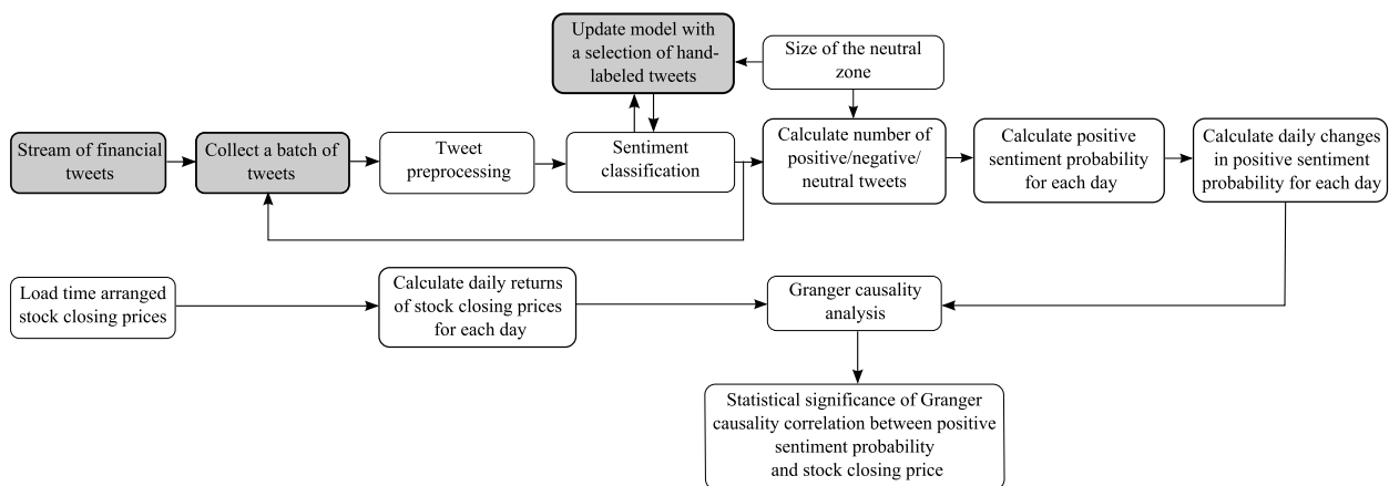
Figure 7: Methodological steps for stream-based active learning for Twitter sentiment analysis in finance. Components which are specific to the stream-based setting and not present in the static setting (Figure 2) are colored gray.
