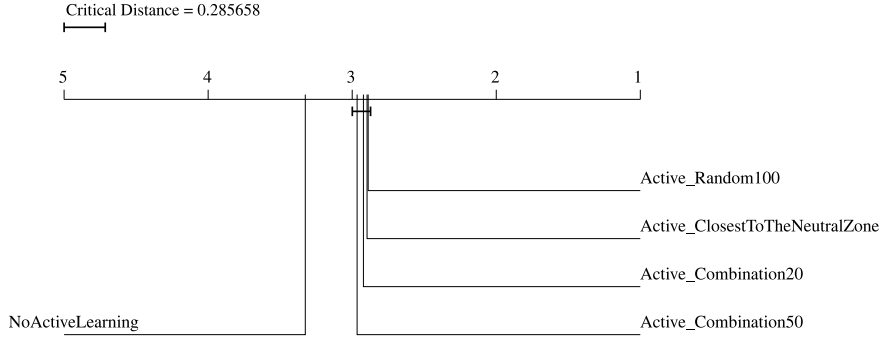
Figure 5: Visualization of Nemenyi post-hoc tests for the “Select 10 of 100” batch selection.
