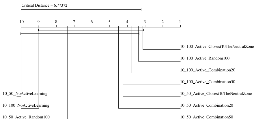
Figure 3: Visualisation of Nemenyi post-hoc tests for the active learning strategies on data from Table 4.
