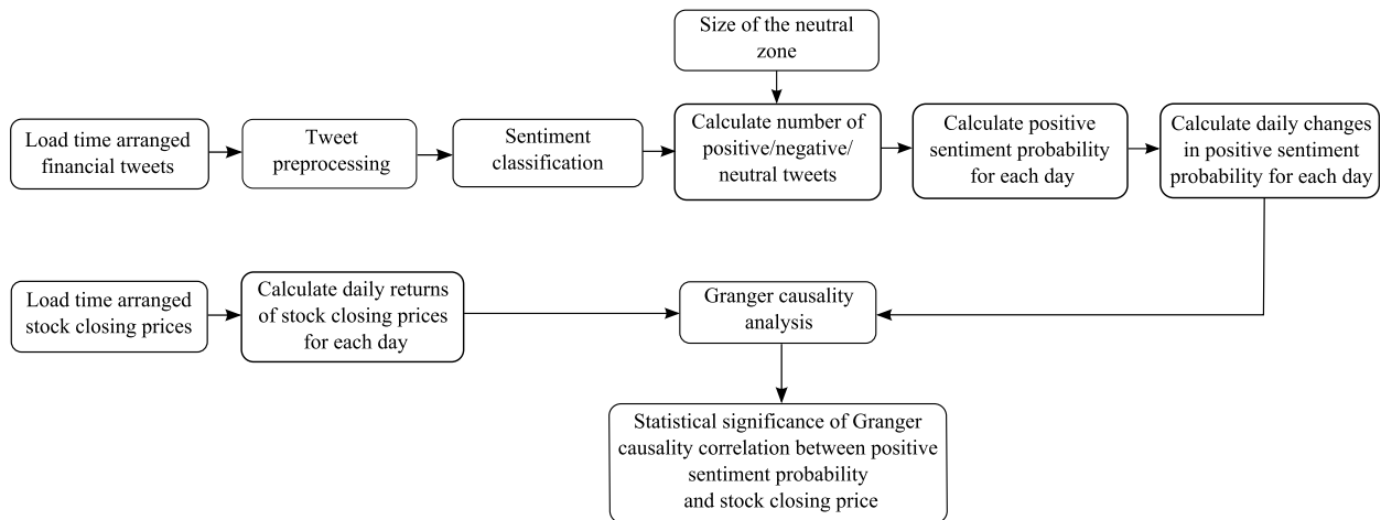
Figure 2: Methodological steps for predictive sentiment analysis applied to determine the correlation between tweets sentiment and stock closing prices.
