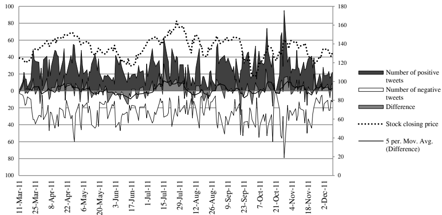
Figure 8: Number of tweet posts classified as positive or negative, their difference, the moving average of the difference (averaged over 5 days), and the stock closing price per day for Baidu.
