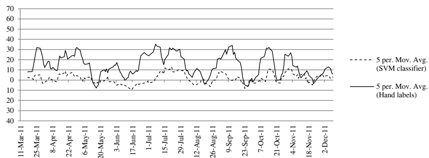
Figure 10: The moving average of the difference (averaged over 5 days) for hand-labeled positive and negative tweets and the ones classified as positive or negative by the SVM sentiment classifier.
