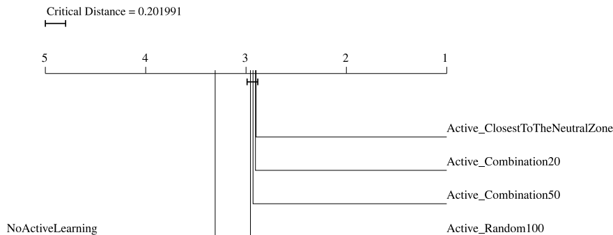
Figure 4: Visualization of Nemenyi post-hoc tests for the “Select 10 of 50” batch selection.
