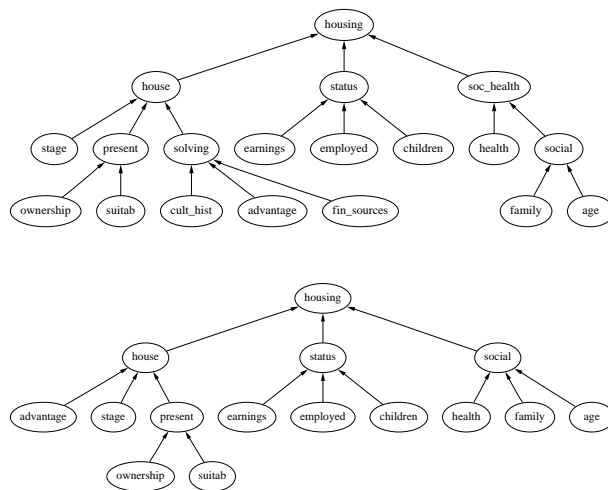
Figure 2: Original (top) and discovered (bottom) concept hierarchy for housing loans allocation.
